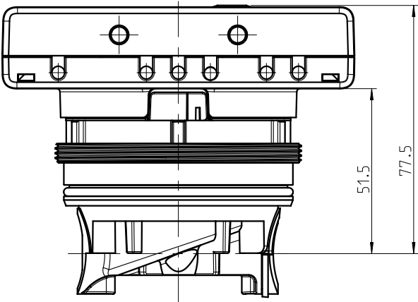
SensoStar 3 multi-jet AStar / compact
