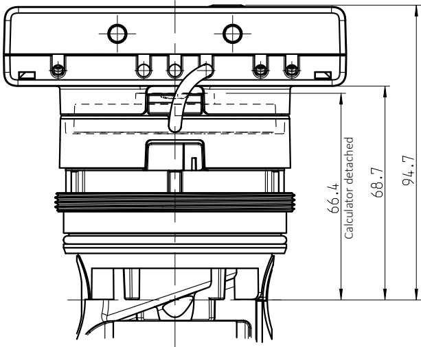
SensoStar 3 multi-jet AStar / split
